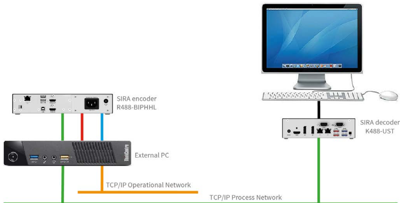
Figure 1: Standalone remote IP configuration - Single session mode with SIRA decoder
