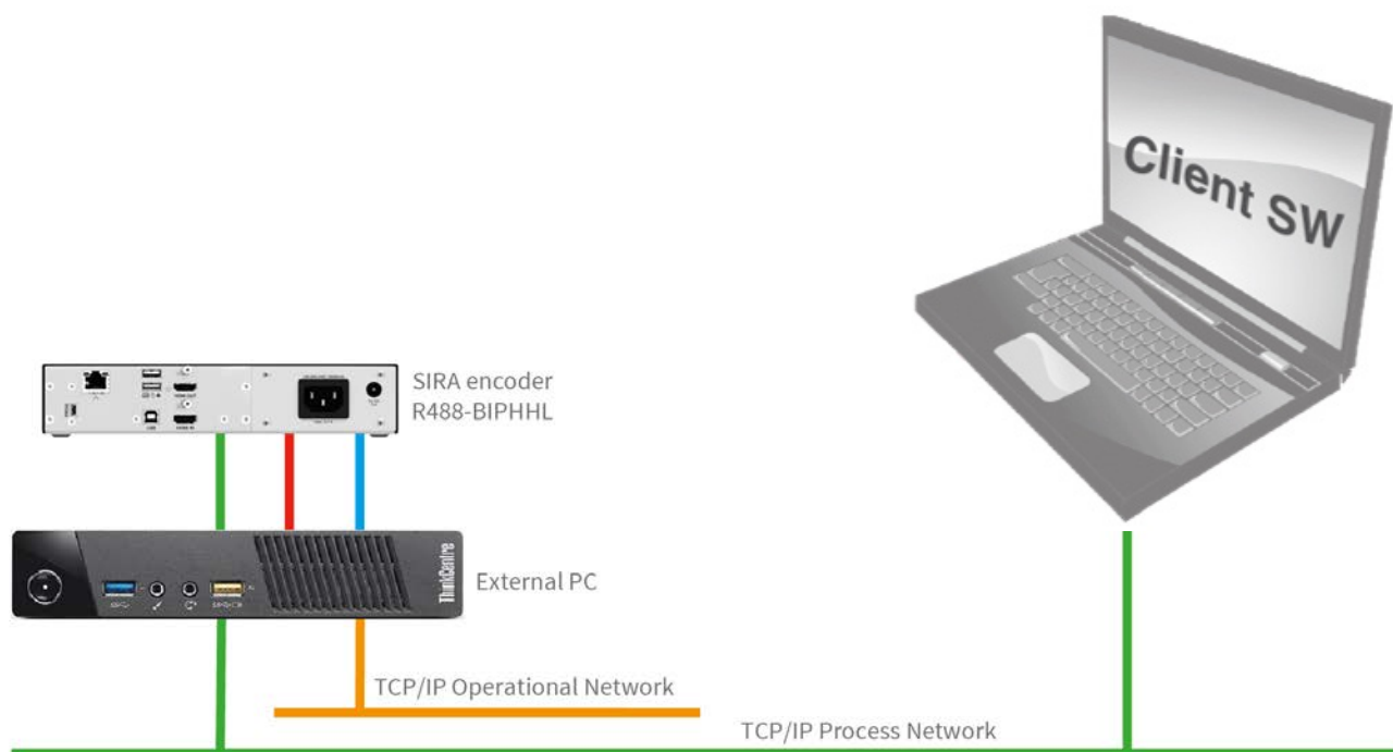
Figure 2: Standalone remote IP configuration - Single session mode with software decoder
